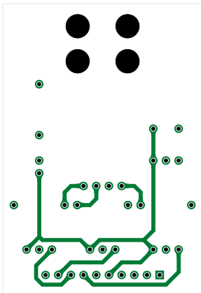
L1 (Top Layer)
