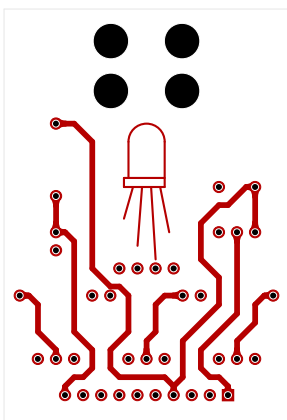
L2 (Bottom Layer)
